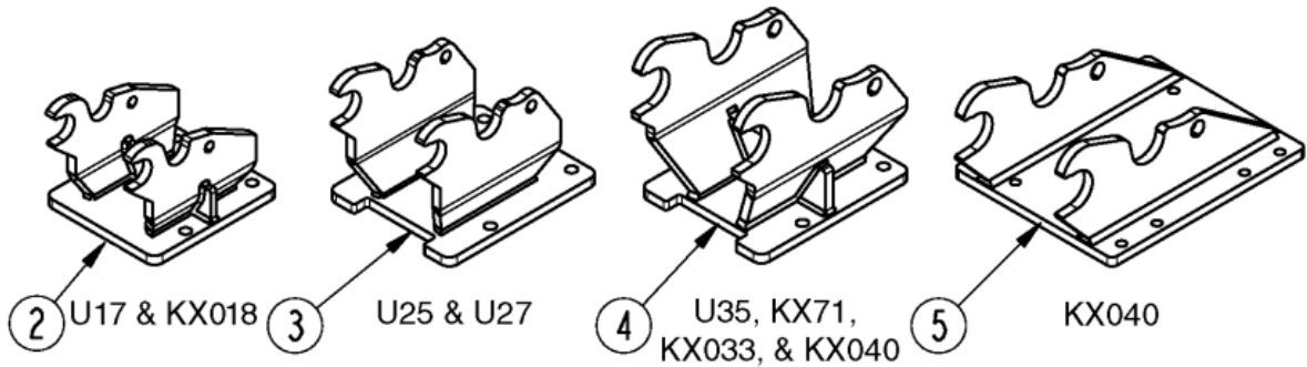
Quick Coupler Mounts for Excavators with Quick attach Couplers
