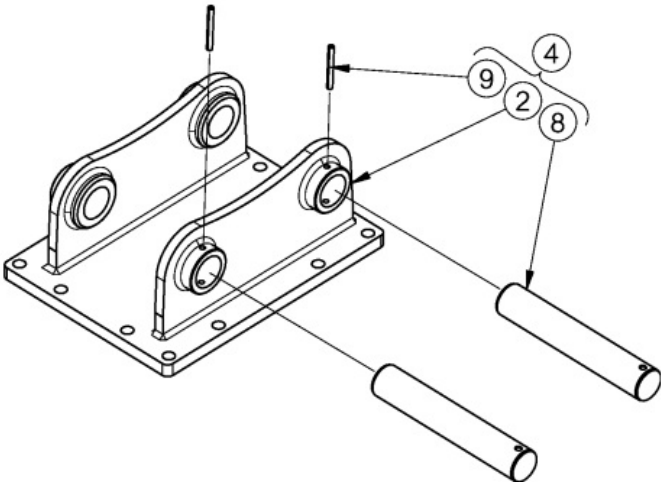
317-442A Pin Grabber Mount : KX080 (BR860)
