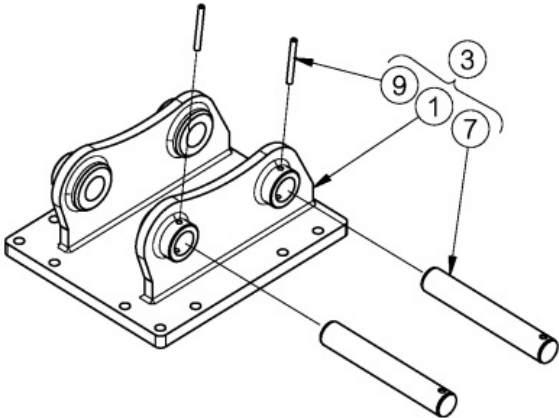
317-441A Pin Grabber Mount : KX057 (BR510 & BR560)
