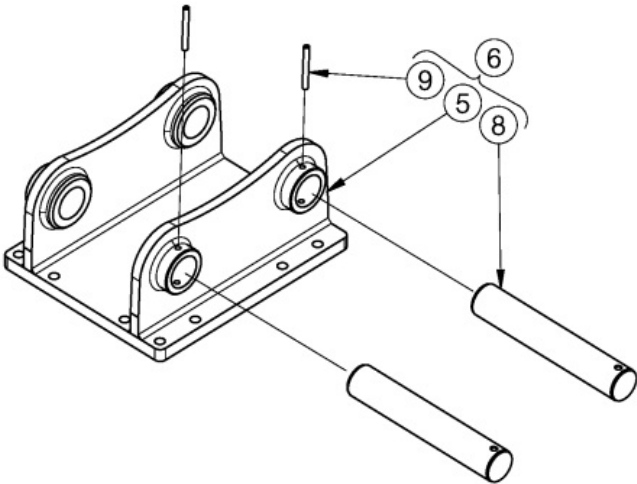
317-444A Pin Grabber Mount : KX080 (BR560)
