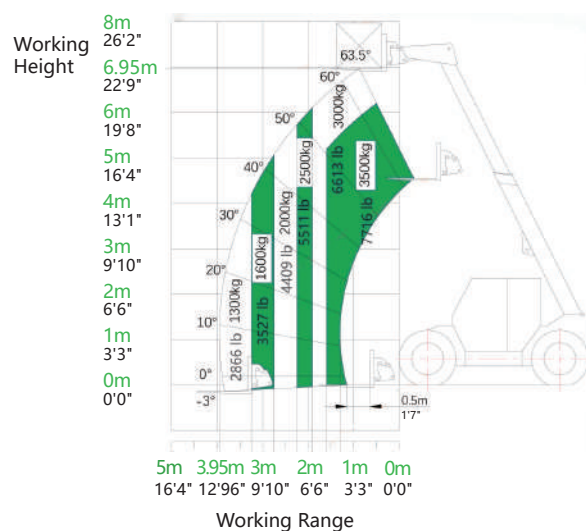
LTH0735E Performance Curve
