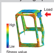
ROPS stress analysis graph
